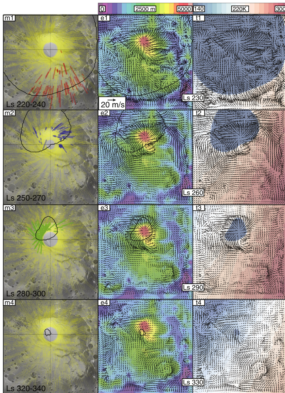
Fig. 8. Maps of SPLD for cloud detections, wind speeds corresponding to topography and temperature. m1–m4: Cloud detections (in red, blue, and green) overlaying available THEMIS image footprints (yellow). For these date ranges, a plethora of observations are available (yellow), and detections of clouds are not limited by spatial coverage. A strong poleward progression of cloud is detected as time of year increases. Solid black line corresponds to the crocus line, or line of CO 2 seasonal ice extent. e1–e4: Map of SPLD wind vectors 20 m above the surface overlaying colorized topography. Winds generally have higher velocities near strong slopes. t1–t4: Map of SPLD wind vectors 20 m above the surface and surface temperature. As the season progresses (L s 230°, 260°, 290°, and 330°) CO 2 seasonal ice retreats (seen in blue with surface temperature ~150 K) (Titus, 2005). The highest wind speeds on the pole are found near the greatest temperature contrast, at the crocus line. Basemap same as Fig. 1a.
