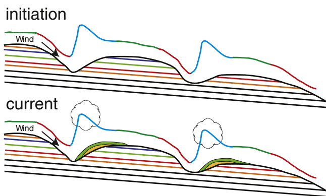
Fig. 15. Cartoon depiction of SPLD trough development. Top: troughs were cut into existing deposits as cycle steps, leaving layered terrain on both sides. Katabatic jumps are required to form the cycle, but water vapor was insufficient for clouds to form, and no material was deposited on the trough low side. Bottom: When conditions became favorable for trough clouds to form, deposition in Australe Lingula and Australe Mensa fully or partially infilled the troughs. Troughs in Promethei Lingula are closer to their initiation state than elsewhere on the SPLD.
