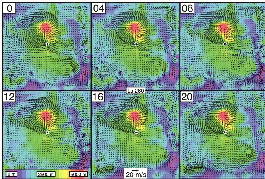
Fig. 7. LMD mesoscale simulations at L_s 260° of wind speed and direction 20 m above the surface. Each panel represents winds at 0° E longitude local time (0–20 h) overlaying colorized terrain. Winds exhibit a diurnal cycle in intensity. Fastest winds are found within and just outside of the crocus line (the extent of the CO_2 seasonal cap as seen in Fig. 8). At this date fast winds are funneled near the wirebrush terrain (at star) throughout the entire day and parallel to erosional scours.
