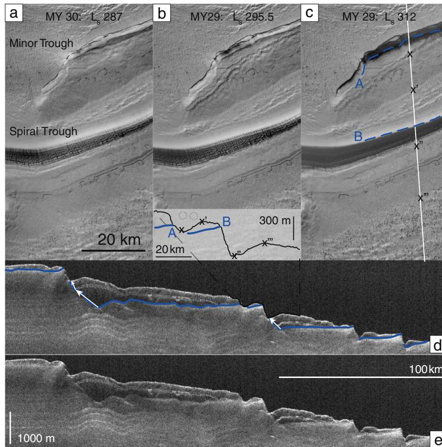
Fig. 5. Observations in Australe Mensa. a) CTX image G11_022371_0932_XL_86S057W at L_s 287 showing minor and major troughs, localized Swiss cheese terrain, and trough clouds. b) CTX image B11_013734_0932_XL_86S057W, similar to a) but at L_s 295.5. c) CTX image B11_014090_0932_XL_86S057W at L_s 312. In each image undular clouds are found at the minor troughs (changing slightly between dates) but not at the major trough. Seasonal frost is reduced on trough high sides as the season progresses. Contact of overlying RFZ 3 and underlying water ice is shown with blue dashed line. White line in c) corresponds to ground track of inset and d), and inset is blow up of interpretation from d). d) Portion of radargram 2579301. RFZ 3 is distinct from lower water-ice deposits (contact in solid blue line). Troughs were filled in during deposition of CO 2 ice and have migrated 10s of kms during a small amount of accumulation (white arrows). e) Uninterpreted radargram 2579301. (For interpretation of the references to color in this figure legend, the reader is referred to the web version of this article.)
