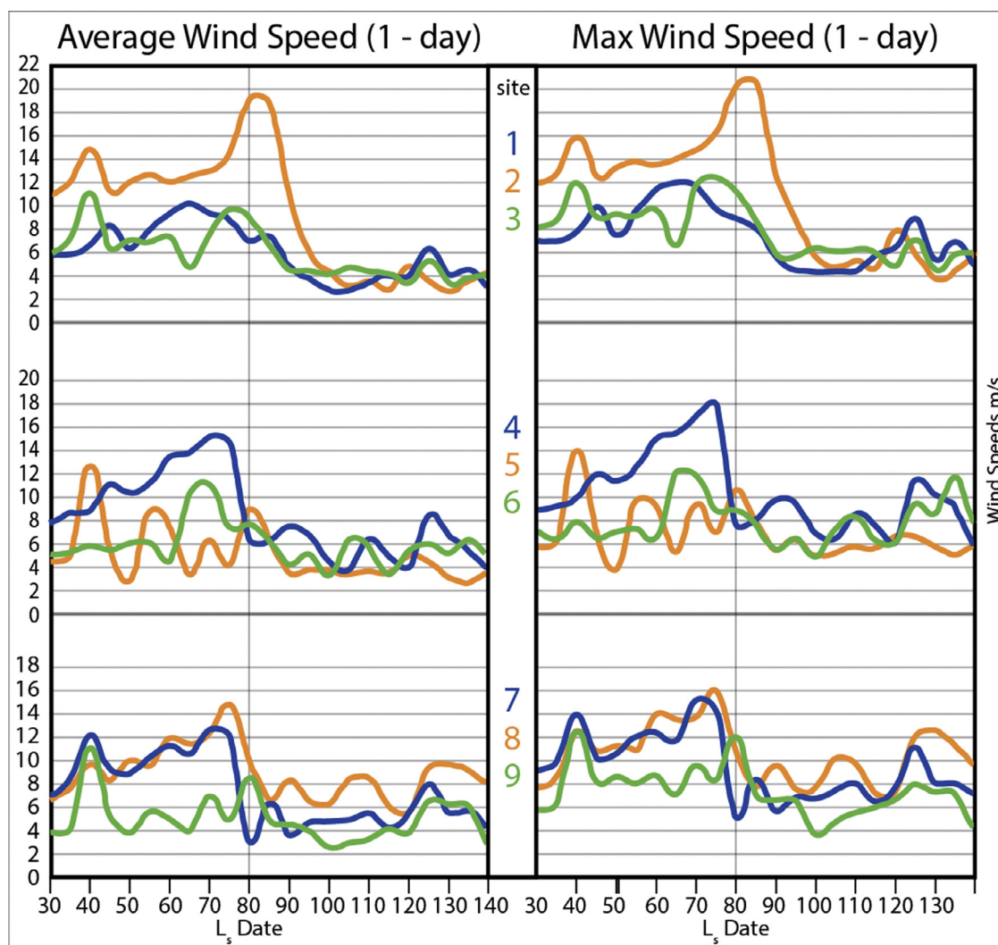
Fig. 4. Average and maximum regional wind speeds 20m above the surface for the final day at each date of our simulation. Wind speeds pick up during spring, as the seasonal cap retreats (Fig. 2). After the crocus line passes each location the speeds drop by a factor of 2–5x. Locations match those in Fig. 3. The cause of the anomalously high wind speeds at L_s 40° are not explained in these simulations.
