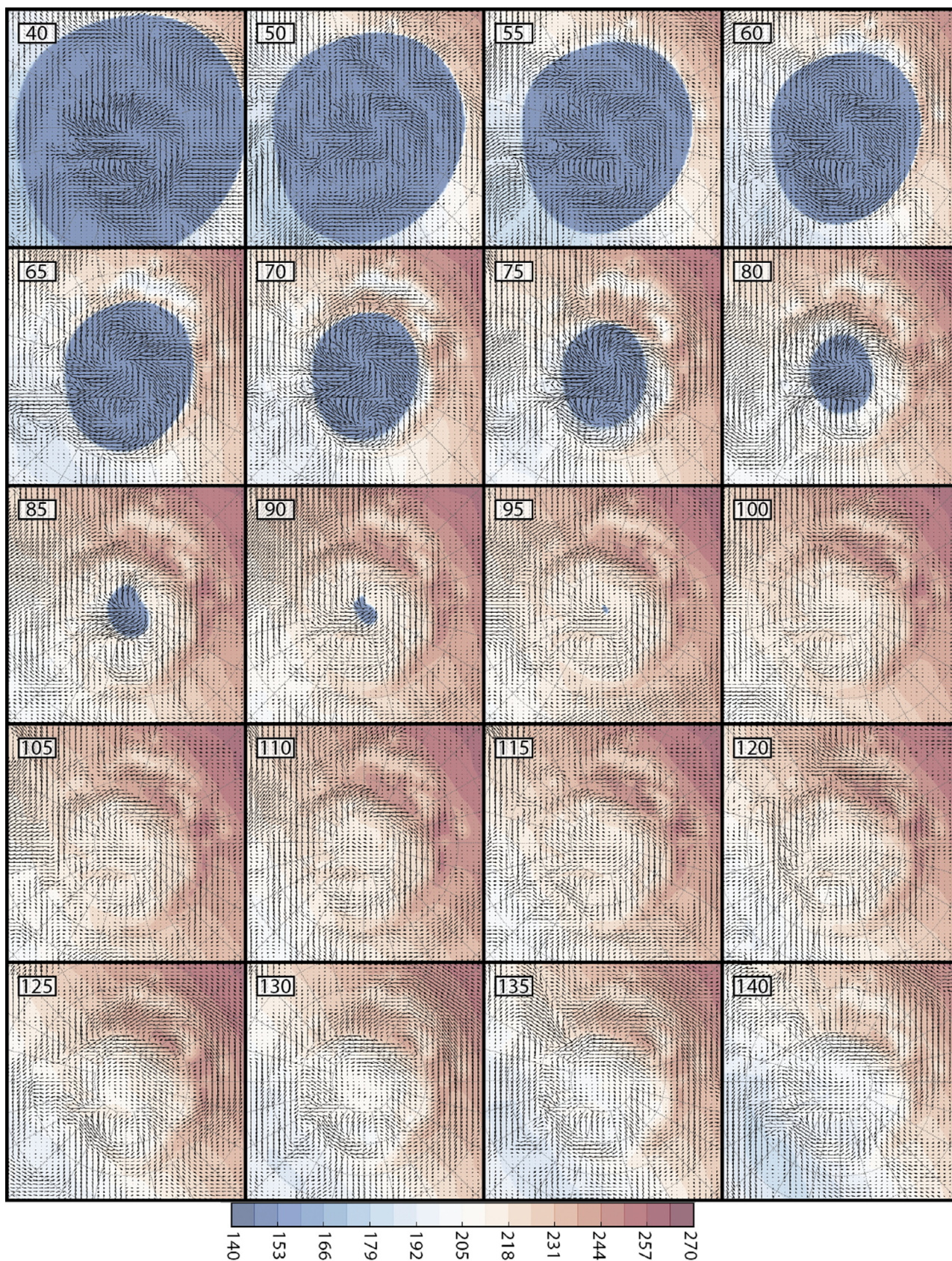
Fig. 2. Model output showing surface temperature (in K) and wind directions 20 m above the surface for most dates in our simulation ( L_s 40°–140°). The \text{CO}_2 seasonal cap dominates the surface thermal environment, and thermal contrasts of 100 K sometimes appear over very short distances. After \sim L_s 95° the seasonal cap disappears, and the surface winds are much weaker (Fig. 4).
