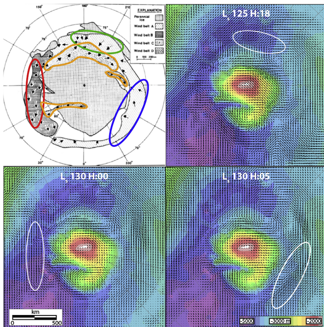
Fig. 7. Comparison of inferred dune migration (a) (Tsoar et al., 1999) to model outputs (b)–(d) Dune fields highlighted in orange align well to the modeled diurnal winds in spring, but other dune fields orient differently. (For interpretation of the references to colour in this figure legend, the reader is referred to the web version of this article.)
